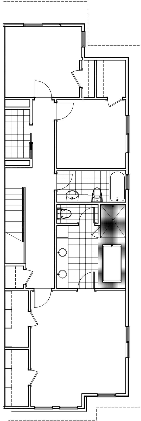
2nd Floor
