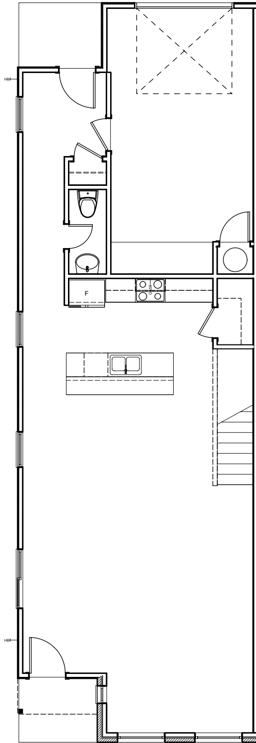
1st Floor
